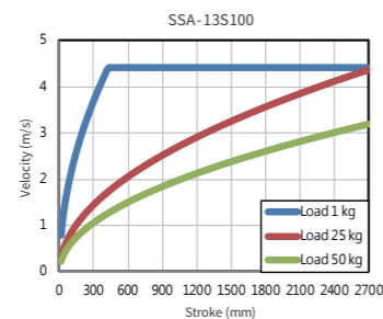
Velocity-Stroke Curve
