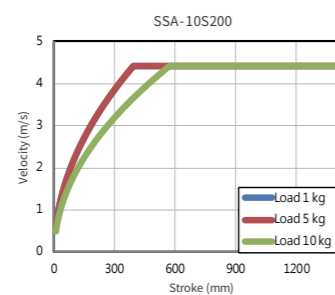
Velocity-Stroke Curve
