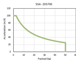
Acceleration-Payload Curve
