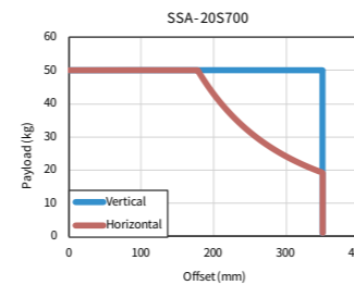
Offset Load Capacity Curve
