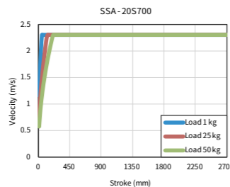
Velocity-Stroke Curve
