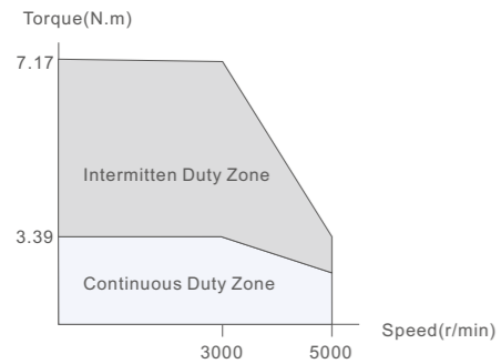
750W Motor
