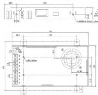
SPS3611(V2.0)/SPS488(V2.0)/SPS607(V2.0)
