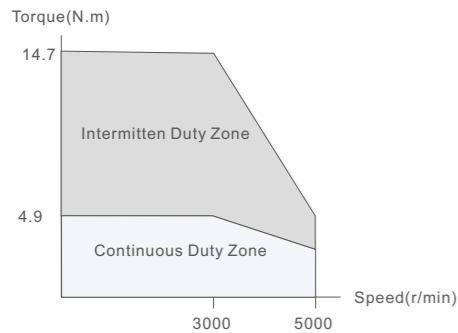
1500W Motor
